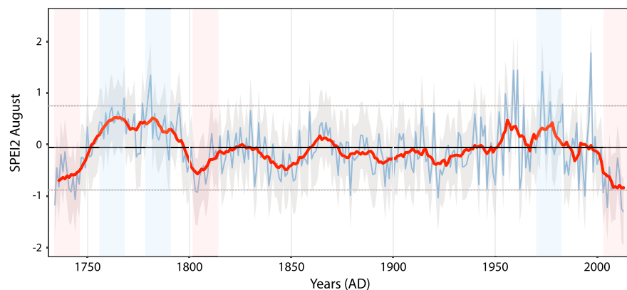
Figure 3. EBSDR reconstruction from 1734 to 2013 for the northeastern Iberian Peninsula. The blue curve represents the reconstruction, the bold red curve is an 11 year running mean, and gray shading indicates the mean square error based on the full calibration correlation period. Vertical shading indicates the extremely wet (in blue) and dry (in red) periods. Dashed lines indicate \pm 1.5 standard deviations (threshold to identify extremely wet and dry events).
