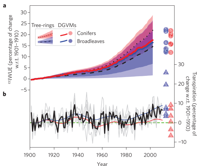
Figure 3 | Water-use efficiency and transpiration variability relative to 1901–1910. Temporal changes in the twentieth century European water balance. a , c_i WUE upper and lower deciles (light shaded), the 22nd and 78th percentiles (dark shaded), and median estimates (dashed) for the broadleaf and conifer sites until 2002. Ensemble means for the DGVM modelled i WUE changes for PFTs (solid lines) together with decadal mean values around 2002 (circles: 1 = CLM4CN; 2 = LPJ; 3 = LPJ-GUESS; 4 = SDGVM; 5 = TRIFFID; 6 = ORCHIDEE). b , Changes in transpiration for the European tree PFTs for the six ensemble members (grey), their mean (black), and for the smoothed broadleaf (blue) and coniferous evergreen (red) ensemble means. Coloured triangles as in a for 2001–2010.
