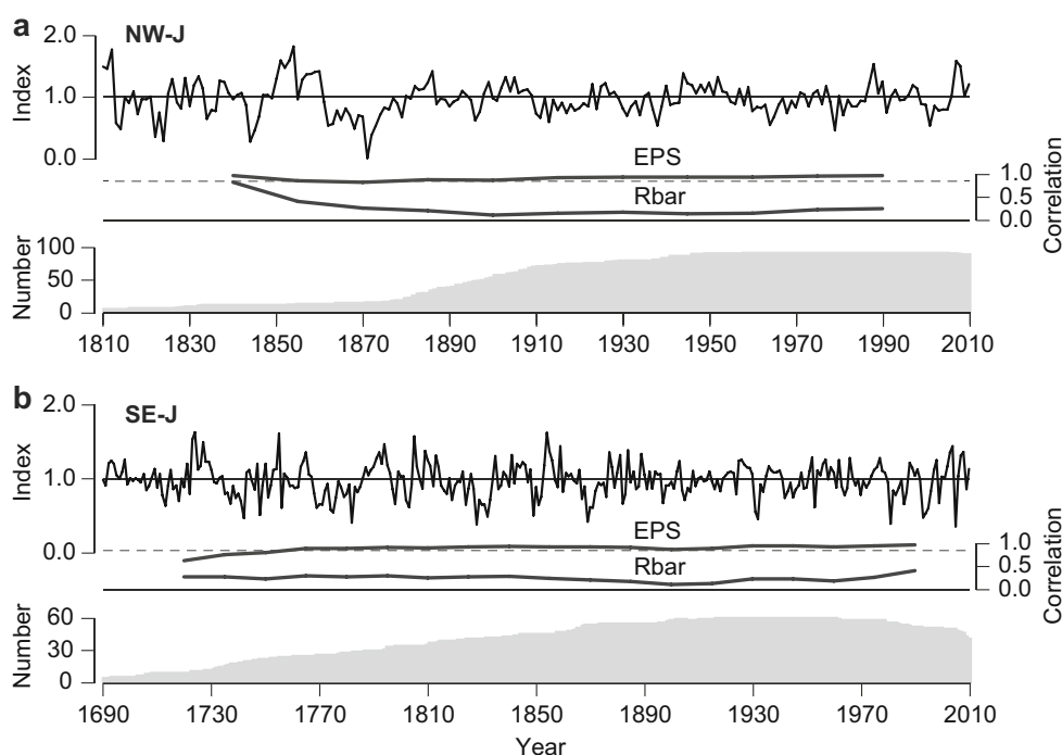
Fig. 2 Juniperus thurifera site chronology characteristics. a The 100-spline detrended NW-J chronology (top panel) shown together with the temporally changing expressed population signal (EPS) and inter-series correlation ( R_{bar} ) and the number of TRW measurement series included in the chronology (bottom panel). b Same as in (a) but for the SE-J data. Dashed lines indicate EPS=0.85 above which a chronology might contain some predictive skill
