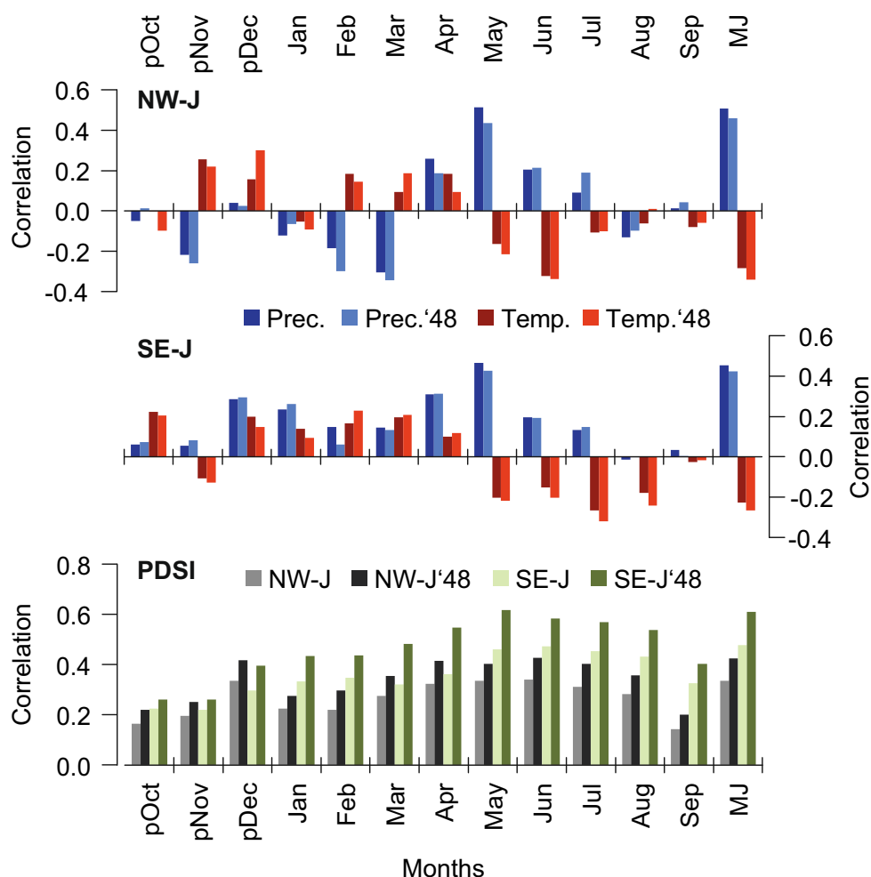
Fig. 3 Climate signals in northwestern and southeastern central Spanish juniper growth. Correlation coefficients between monthly precipitation (blue) and temperature data (red) with NW-J and SE-J tree ring width data (top and middle panels). Bottom panel shows correlations with gridded PDSI data (gray and green). All correlations are computed over the (full) periods of overlap with instrumental data (see Table 1: 1944–2010 for Soria, 1948–2003 for Teruel, 1901–2002 for gridded PDSI) as well as over the period 1948–2002 common to all instrumental records (labeled '48 in the figure). Bars for pOct, pNov, and pDec indicate correlations with previous year's months. MJ is a seasonal mean integrating May and June data. For the common-period calculations, p < 0.05 is reached at r \approx 0.3
