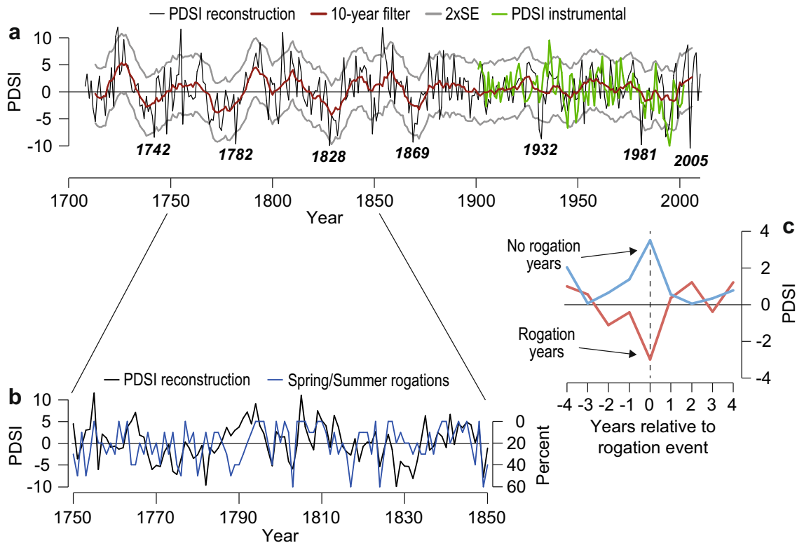
Fig. 6 PDSI reconstruction and comparison with rogarion ceremony data. a Annually resolved PDSI reconstruction back to 1708 (black curve), derived from scaling the SE-J chronology against instrumental PDSI data (green), shown together with a 10-year filter (red). Uncertainty is estimated considering the standard error (2xSE, gray) of the calibration model from 1948–2002. Seven reconstructed driest years exceeding
