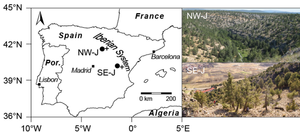
Fig. 1 Juniperus thurifera sampling sites in northwestern (NW-J) and southeastern (SE-J) Iberian System. Crosses indicate climate stations in Soria near NW-J and Teruel near SE-J
