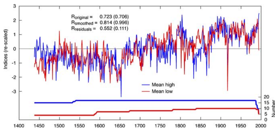
Fig. 4 Comparison of the high- ( blue ) and low-elevation ( red ) composite mean chronologies from western central Asian juniper sites. The series are shown back to 1438, where Mean low reached four site chronologies ( lower panel ). Correlations refer to the 1438–1995 period
