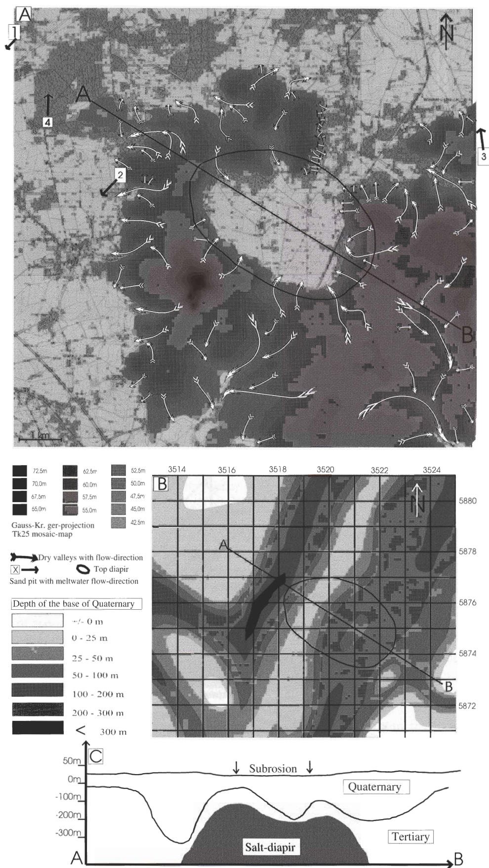
Fig. 6. a) Topographic height around the Wedehof diapir with flow direction along dry valleys (white arrows) and flow direction of channels (age unknown) in the Saalian meltwater sands. The black oval delineates the top of the diapir. b) Depth of the base of the Quaternary, formed by deep tunnel valleys of Elsterian age. c) Cross section AB over the Wedehof diapir.
