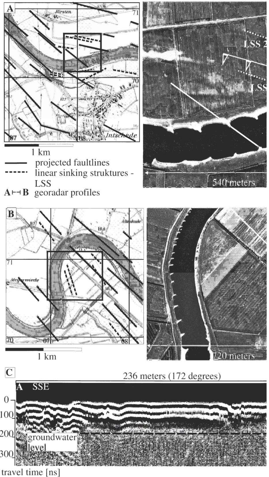
Fig. 5. a, b) Projected (from Fig. 4) fault lines, topographic map and aerial photograph of the river Weser alluvial plain, c) ground penetrating radar (25 MHz) of linear sinking structures (LSS) near to projected fault lines (profile A-B on Fig. 5a).
