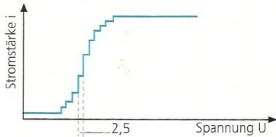
3. Pulse Polarogramme
