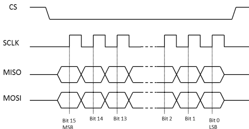
Figure 11. Timing diagram of one word
