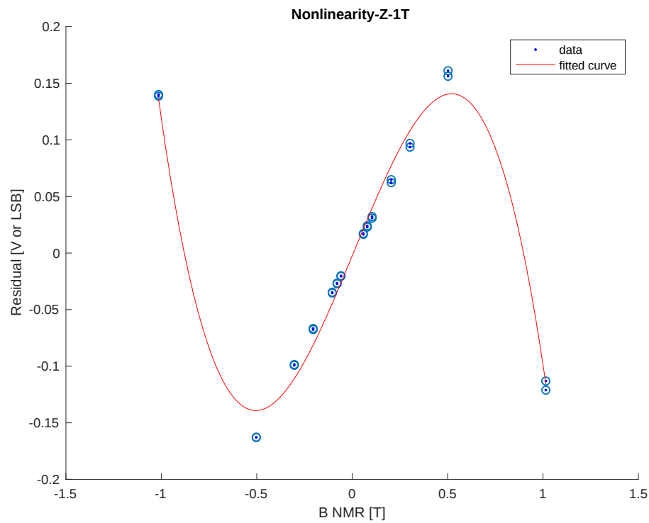
Figure 4. Typical nonlinearity plot, VCC = 3.3 V
