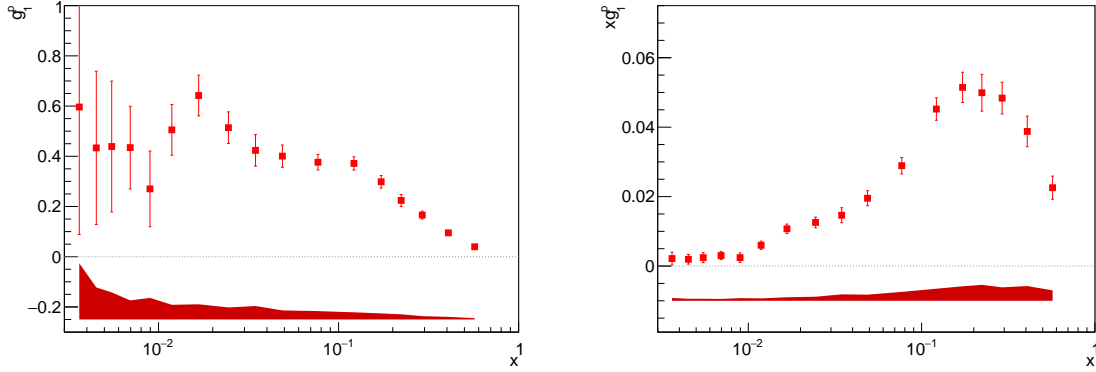
Figure 92: Results for the structure function g_1^p (left) and xg_1^p (right) as a function of x .
