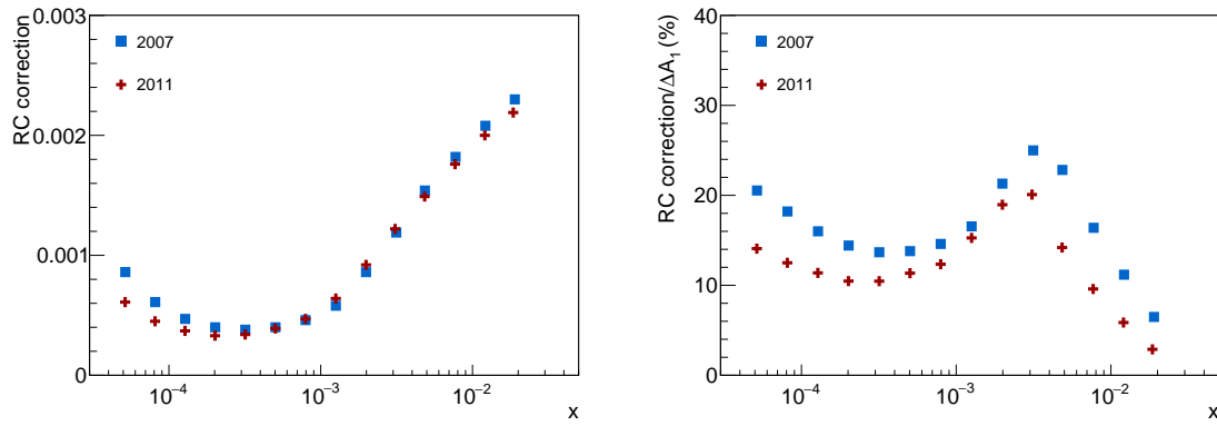
Figure 122: Correction to the asymmetry due to polarised radiative effects in bins of Bjorken- x . Left: absolute size of the correction. Right: Relative size of the correction compared to the statistical uncertainty.
