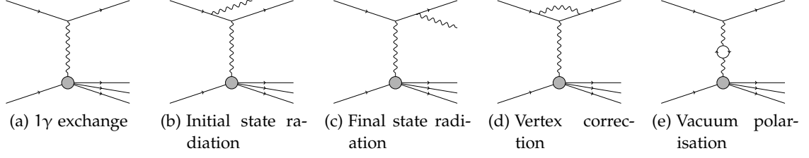
Figure 62: Various processes, which contribute to radiative corrections to the one photon exchange in inclusive deep inelastic scattering.
