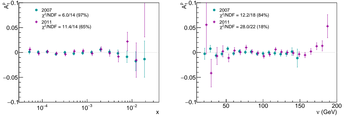
Figure 112: Results for the asymmetry obtained using fake configurations. The results of the 2011 data taking are slightly shifted for better visibility and the \chi^2 for the results from both years to be compatible with zero is given. Left: Results as a function of Bjorken- x . Right: Results as a function of the virtual photon energy.
