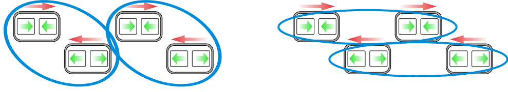
Figure 71: Illustration on how the fake configurations (right) are formed compared to the consecutive ones (left). The green arrows correspond to the polarisation direction of the target cells and the red ones show the direction of the solenoid field. The blue circles illustrate how the groups are formed.
