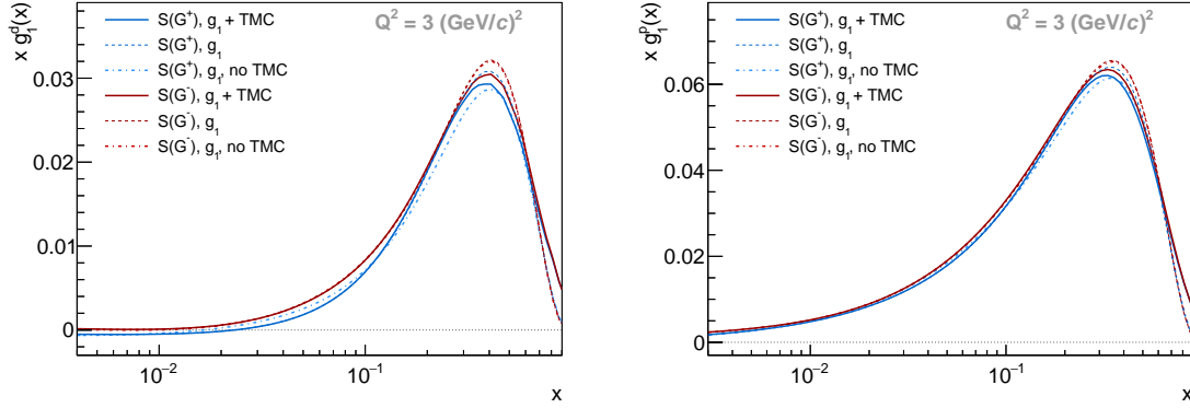
Figure 147: Comparison between the results of the QCD fit without the target mass correction ( g_1 , no TMC) and the results of the QCD fit including the target mass correction for the spin-dependent structure function with ( g_1 + \text{TMC} ) and without ( g_1 ) the correction. Left: Spin-dependent structure function of the deuteron. Right: Spin-dependent structure function of the proton.
