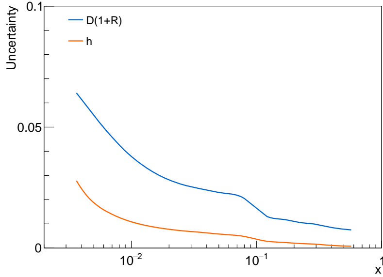
Figure 82: Illustration of the size of the systematic uncertainty from taking into account the uncertainties on the depolarisation factor and the cross section ratio R independently and in a combined way.
