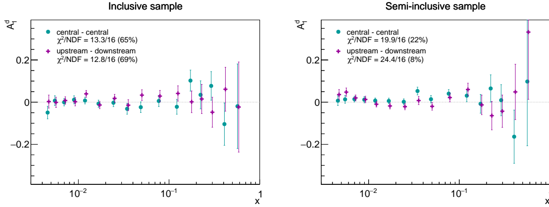
Figure 74: Results for the asymmetries obtained from the 2006 data combining target cells with the same polarisation direction. The results for the combination of the outer cells are slightly shifted for better visibility and the \chi^2 for both samples to be compatible with zero is given. Left: Results for the “inclusive” sample. Right: Result for the “semi-inclusive” sample.
