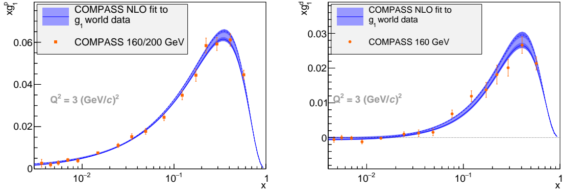
Figure 148: Comparison between the spin-dependent structure function of the proton (left) and deuteron (right) and the results for these structure functions of the QCD fit. The results are shown at a photon virtuality of 3 \text{ (GeV/c)}^2 .
