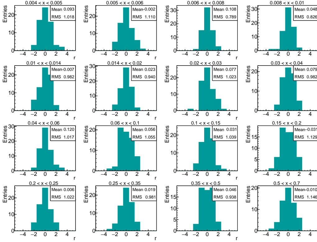
Figure 78: Pulls distributions obtained from the data taken in 2006 for each Bjorken- x bin. The results from the two samples of the 33 periods are shown.
