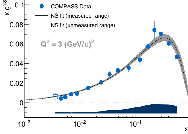
Figure 155: Values of xg_1^{\text{NS}}(x) at Q^2 = 3 (\text{GeV}/c)^2 compared to the non-singlet NLO QCD fit using COMPASS data only. The errors are statistical only. The open square at lowest x is obtained with g_1^d taken from the NLO QCD fit.
