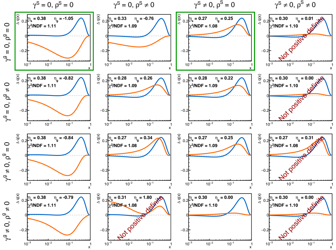
Figure 134: Results of the QCD fit for various functional forms are shown at Q^2 = 3 \text{ (GeV/c)}^2 . The blue curve represents \Delta q^S(x) , the orange one \Delta q^g(x) . The first moment of these distributions at the input scale and the \chi^2 value are given for comparison. The solutions shown in panels one and three of the first row (surrounded by green boxes) represent the two solutions S(G^-) and S(G^+) .
