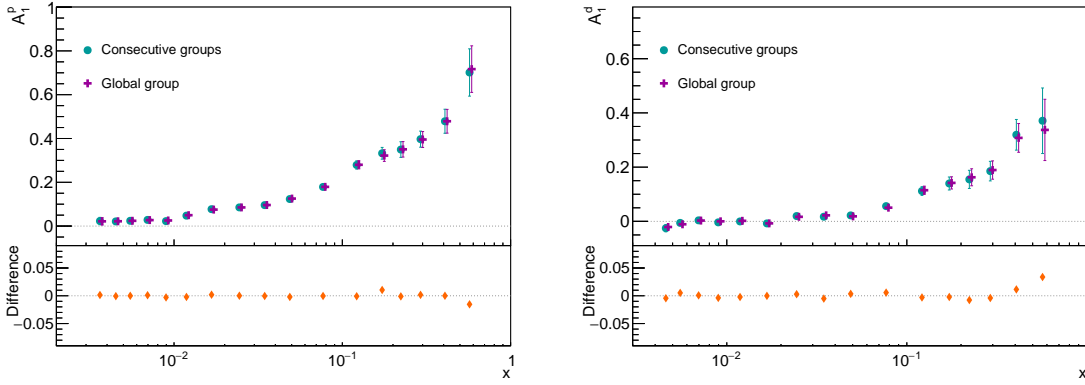
Figure 70: Result for the asymmetry A_1^p (left) obtained from the 2011 data and A_1^d (right) obtained from the 2006 data using two different ways for combining the various periods. The results for the global grouping are slightly shifted for better visibility.
