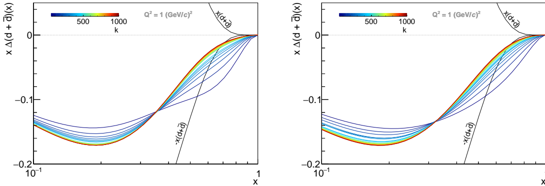
Figure 131: Effect of the increasing strength of the positivity constraint on the down quark helicity distribution. The results are shown at a fixed photon virtuality of Q^2 = 1 \text{ (GeV/c)}^2 for the two solutions of the QCD fit. Left: Solution S(G^-) . Right: Solution S(G^+) .
